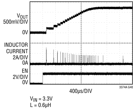
4A Buck Regulator No-Load Start-Up Transient
